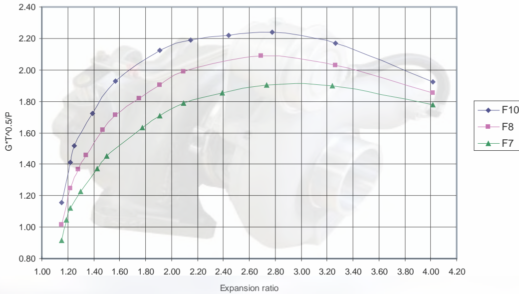
Turbine Maps
